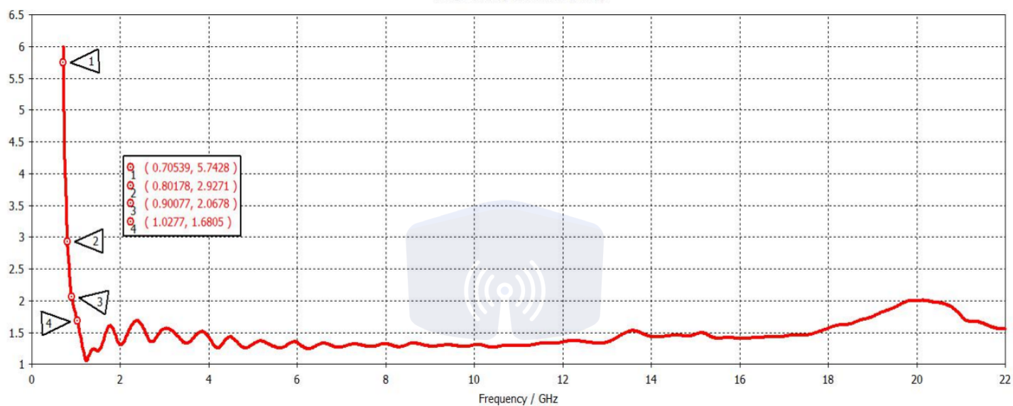
Voltage Standing Wave Ratio (VSWR)
